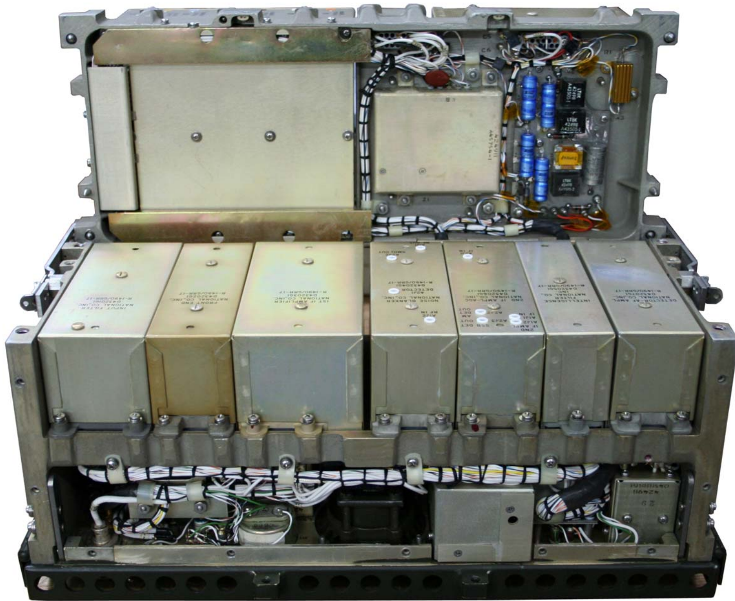
Figure 5-6, Rear Deck A1A3 S/N:466, Bottom View , Refer to Page 5-44
